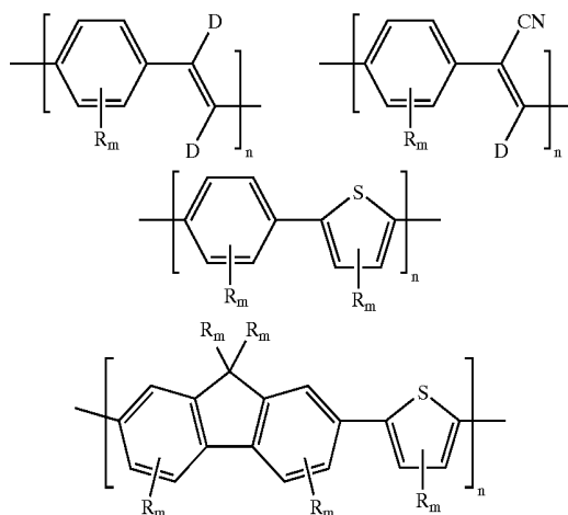
Scheme 5 Organic semiconductor compounds and polymers with deuterium substituents. (R: D, H, C 1 -C 30 alkyl, C 1 -C 30 alkoxy, phenyl, thienyl, pyridyl, C 1 -C 30 silyl, aryl, heteroaryl; m is from 1 to 4).
