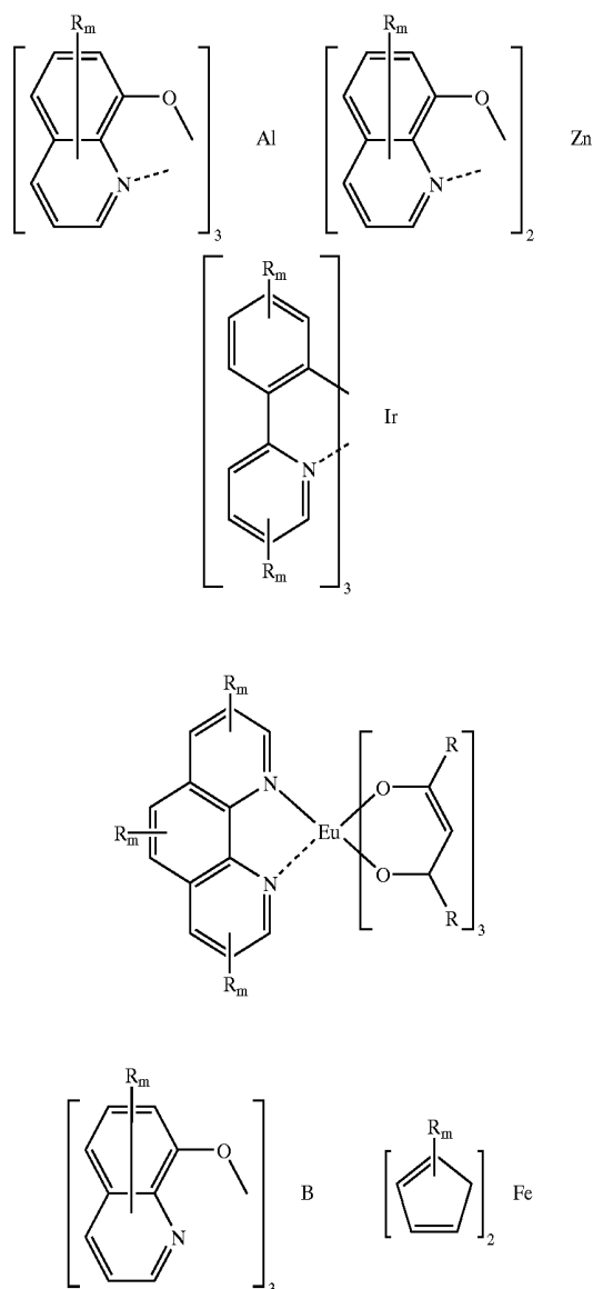
Scheme 4 Metal complexed organo-metallic compounds. (R: D, H, C 1 -C 30 C 1 -C 30 alkoxy, C 1 -C 30 silyl, aryl, heteroaryl; m is 1-4).
