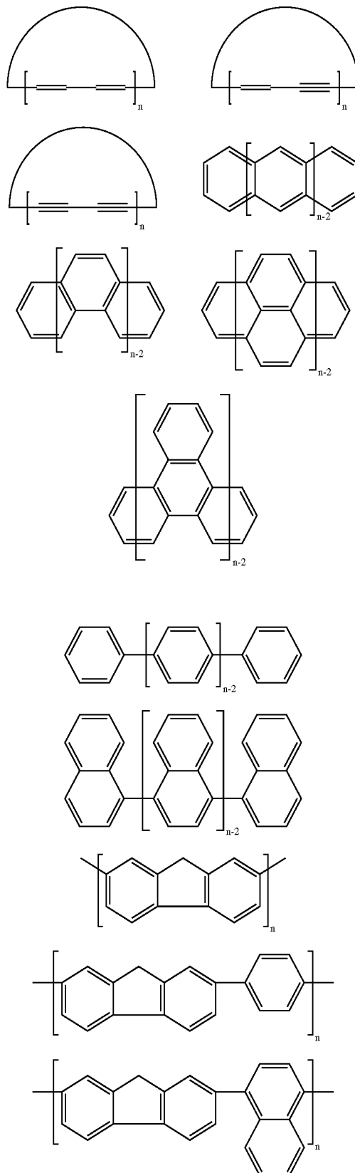
Scheme 2 Cyclic and fused ring combinations
